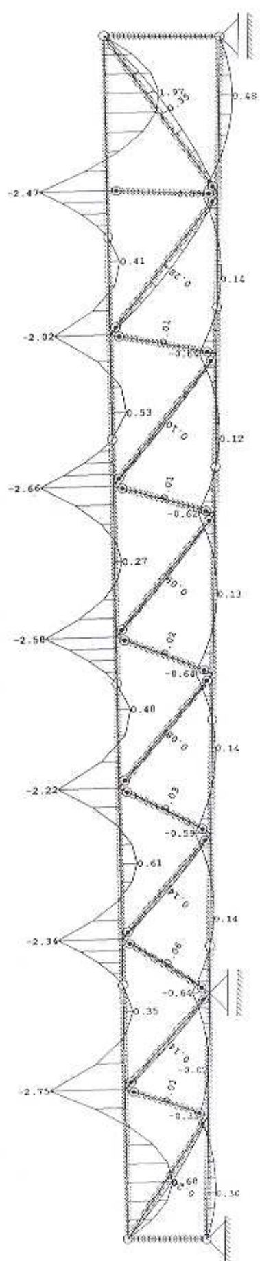
Opt. 4 - Uijecaji u gredi: Mz (kNm)
